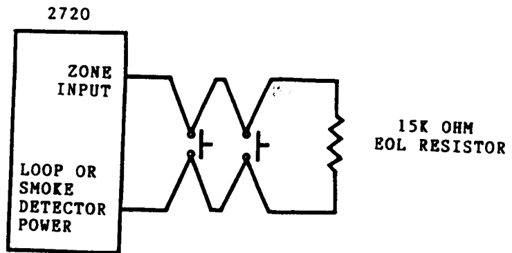
b) Intrusion Zone - using both Normally Open and Normally Closed initiating devices and an End-Of-Line resistor. The Normally Closed and the Normally Open contacts will be supervised; i.e. - an alarm will occur if the loop is crossed or broken.
