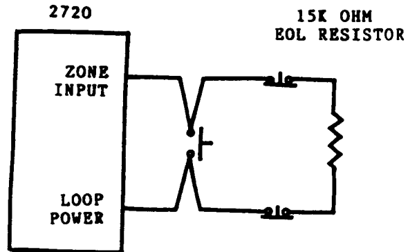
b) Intrusion Zone - using both Normally Open and Normally Closed initiating devices and an End-Of-Line resistor. The Normally Closed and the Normally Open contacts will be supervised; i.e. - an alarm will occur if the loop is crossed or broken.
