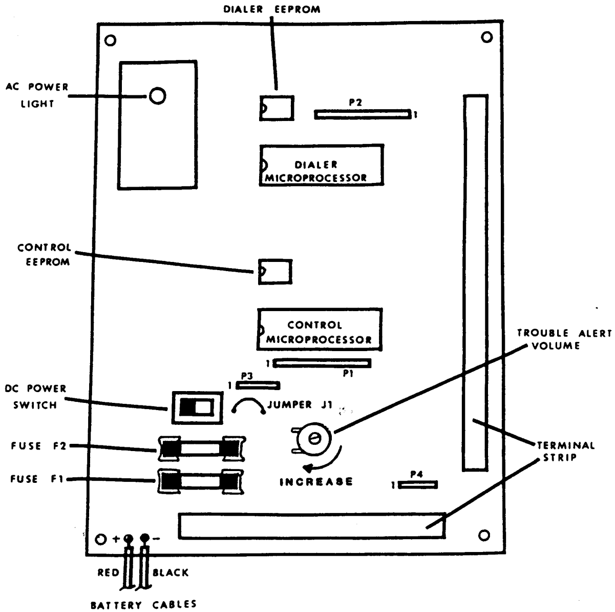
MODEL 2720 CIRCUIT BOARD
