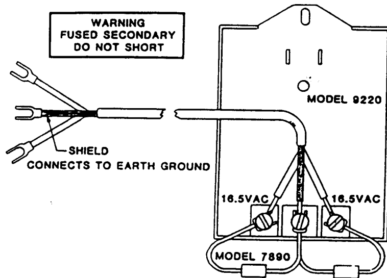
MODEL 9220 TRANSFORMER
