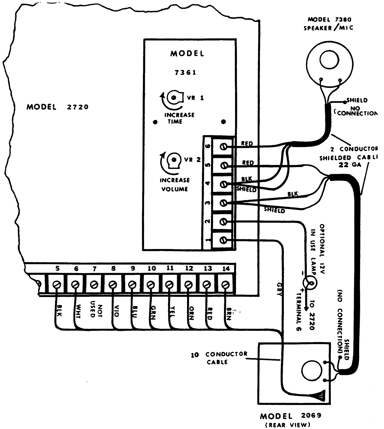
FIGURE 15 MODEL 2720 INTERCOM WIRING
