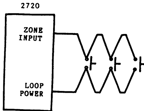
a) Unsupervised Intrusion Zone - using Normally Open contact initiating devices only and no End-Of-Line resistor. NOT ACCEPTABLE FOR UL INSTALLATIONS.
